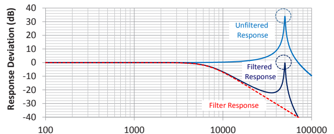
Filtering to Minimize Amplifier Saturation
