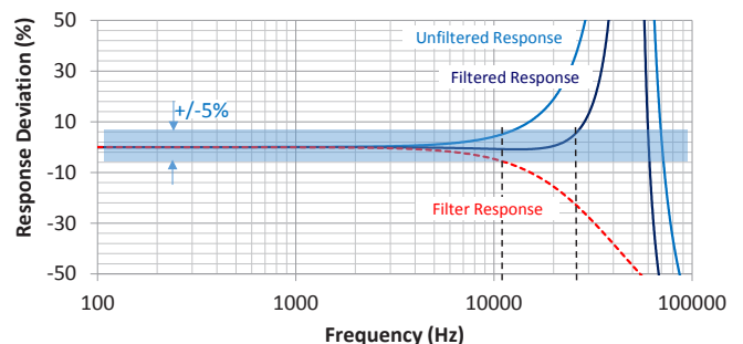
Filtering to Minimize Amplifier Saturation
